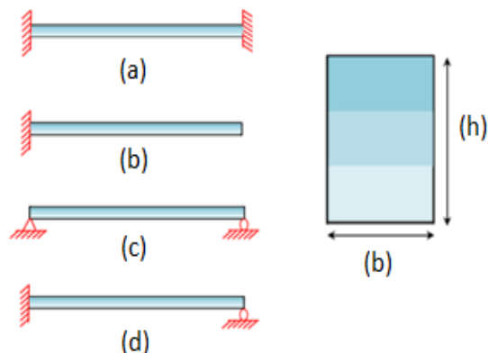
Fig. 1 (a) clamped-clamped, (b) clamped-free, (c) simply supported-simply supported, (d) simply supported-clamped straight uniform nanobeams with rectangular cross-section
